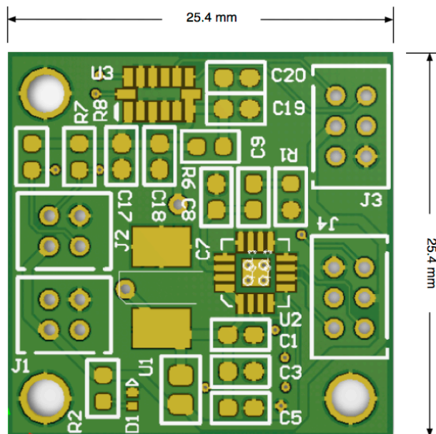
Figure 3 MK-95157 Board Dimensions
