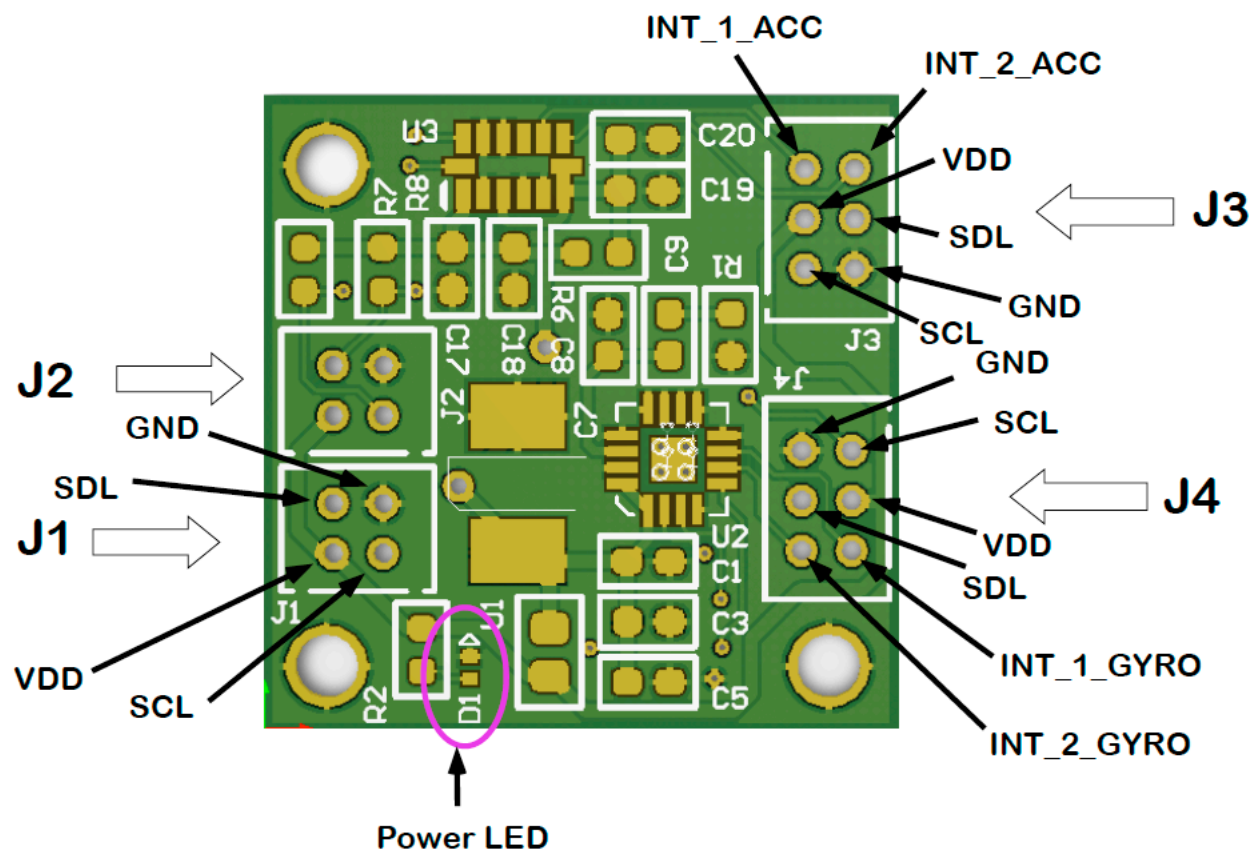
Figure 4 MK-95157 Connections
