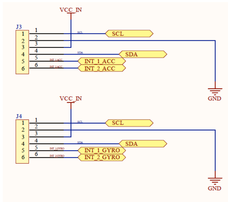
Figure 6 I2C Connections with Interrupts
