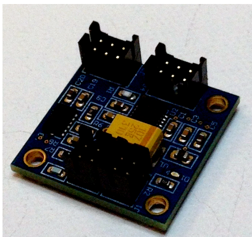
Figure 2 MK-95157 I2C 3-Axis Gyro and 3-Axis Accelerometer Another View
