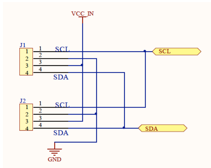
Figure 5 I2C Bus 4 Pin DF11 Hirose Connections
