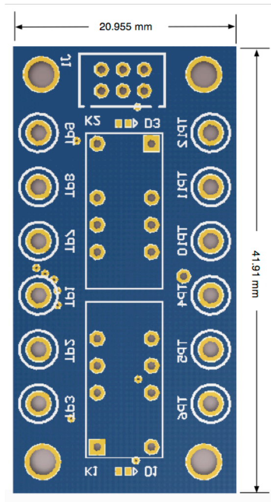
Figure 4 MK- 91648 Board Dimensions
