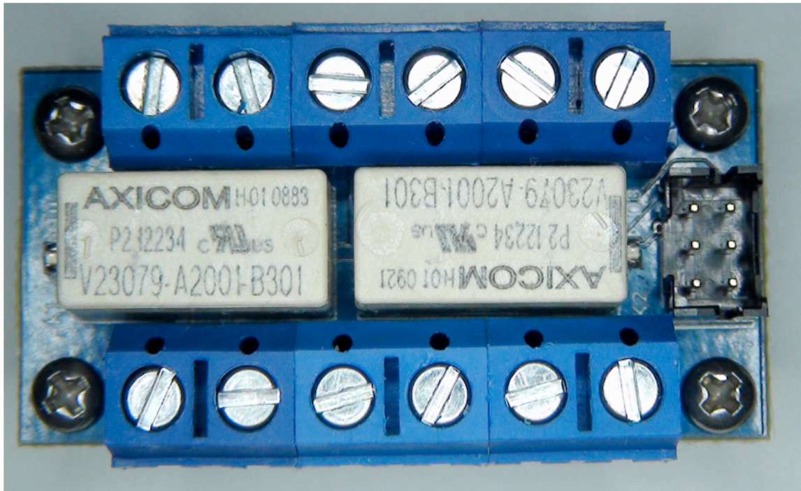
Figure 3 MK- 91648 DUAL SPDT Relay GPIO Control Top View
