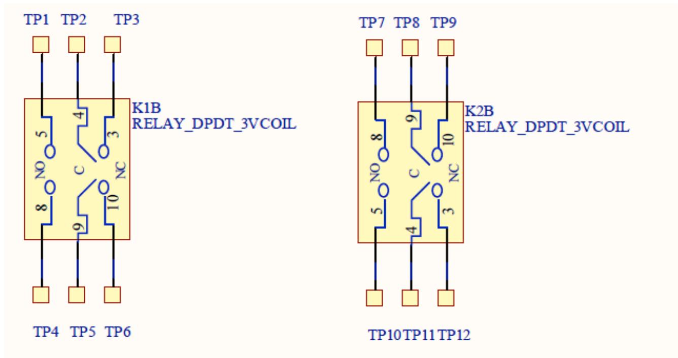
Figure 7 Relay Terminals Schematic
