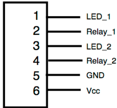
Figure 5 J1 6 Pin DF11 Series Hirose Connector for Relay and LED Control
