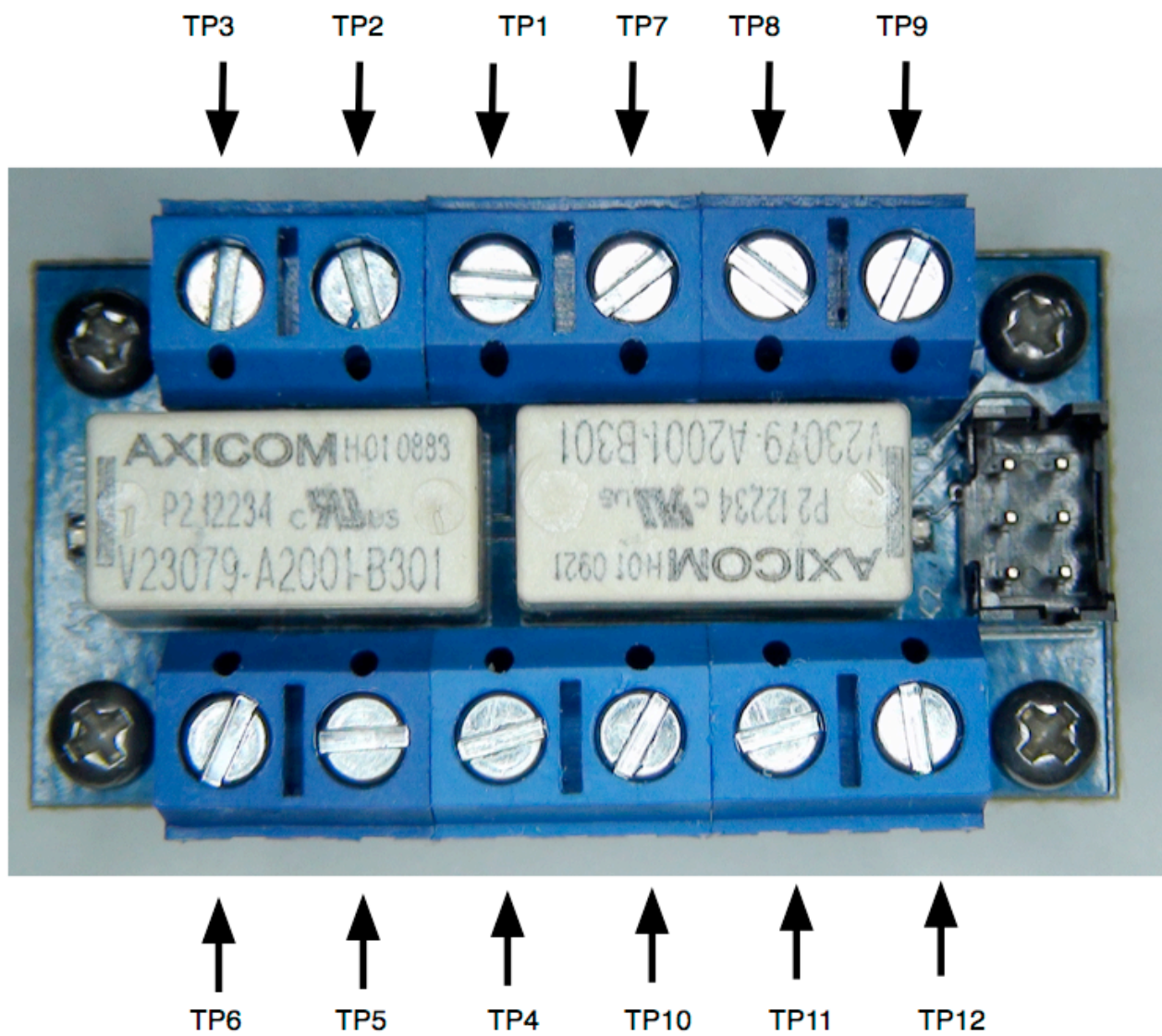
Figure 8 Relay Terminals
