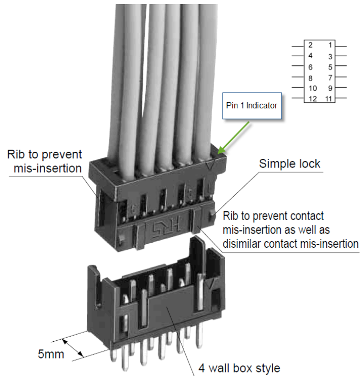
Figure 9 Guide to the Hirose DF11 series connector
