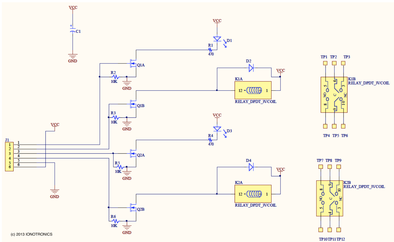
Figure 6 MK-91648 Dual SPDT Relay GPIO Control Schematic
