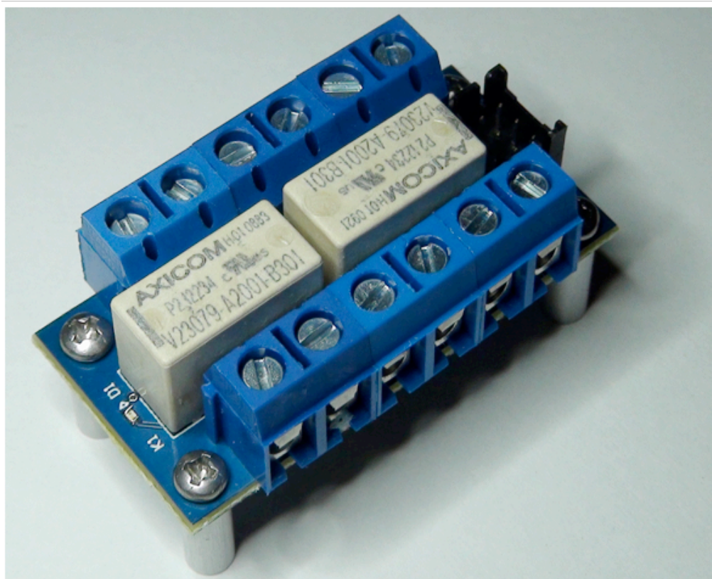
Figure 2 MK- 91648 DUAL SPDT Relay GPIO Control Another View
