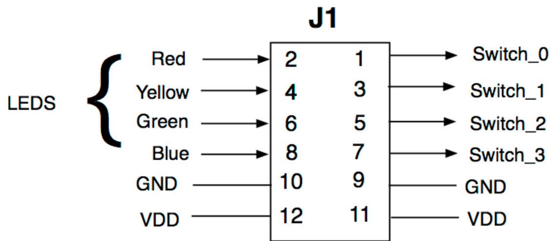
Figure 5 MK-55857 Pin Out
