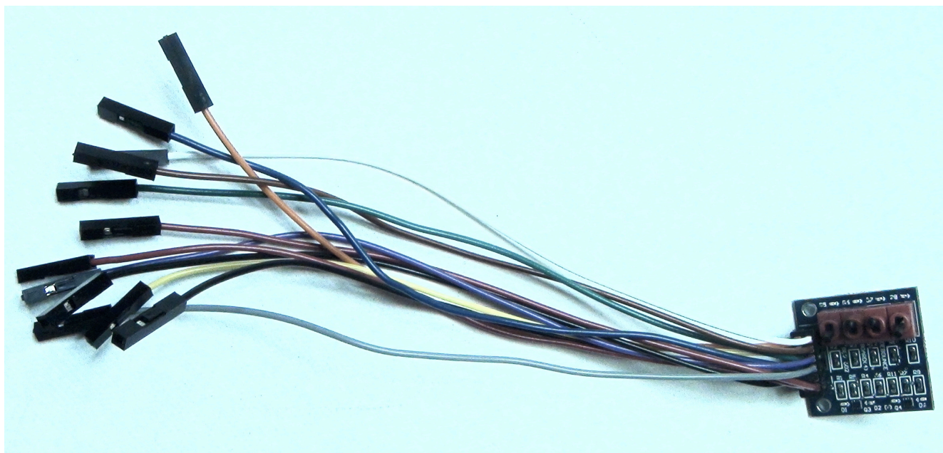
Figure 4 Mk-55857 with DF-11 to 25mil 0.1" Post Cable (MK-89808)
