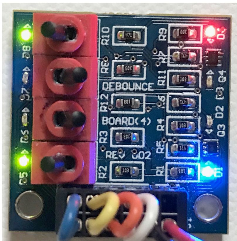
Figure 3 Loop Back Test Switch 0 and 3 On
