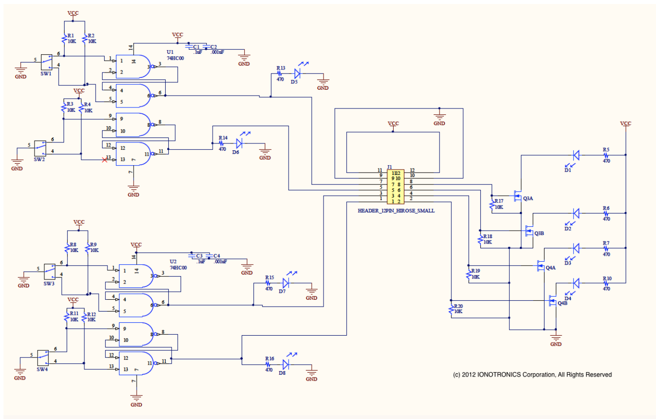
Figure 6 MK-55857 Schematic
