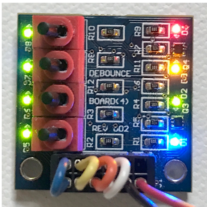
Figure 2 Loop Back test All On
