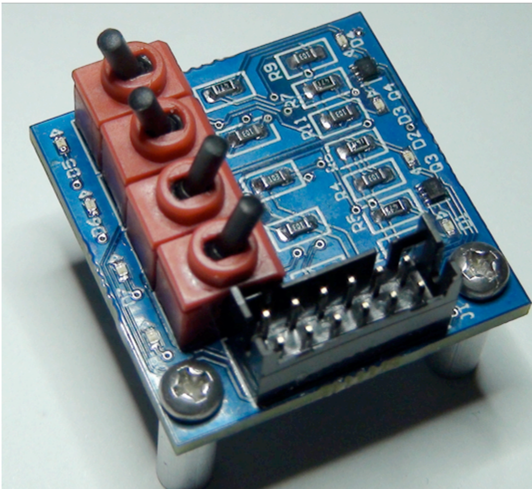
Figure 1 Photo MK-55857 4x Debounce Switch Color LEDs
