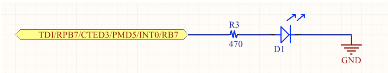
Figure 4 Port RB7 drives an LED that can be used for tests and status
