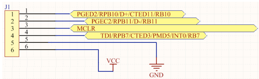
Figure 7 J1 6 Pin Hirose DF11 Series. ICSP (Programming) and GPIO
