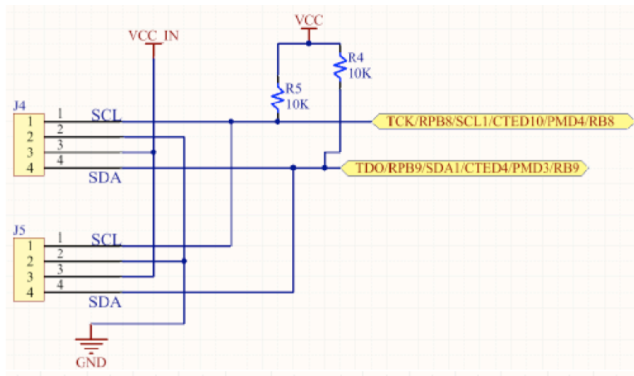
Figure 6 I2C Bus J4 and J5 4 Pin Hirose DF1 Series Connectors
