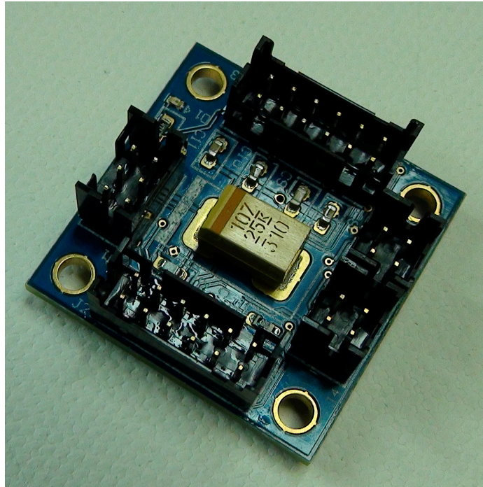
Figure 1 Top view MK-53393 illustrating DF11 Hirose Connectors for GPIO and 4 Pin I2C Bus
