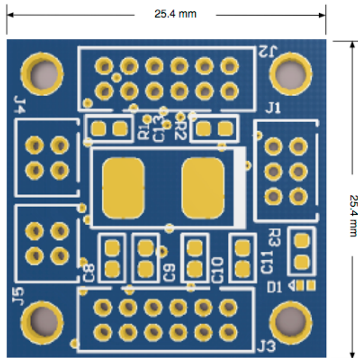
Figure 3 Board Dimensions for the MK-53393
