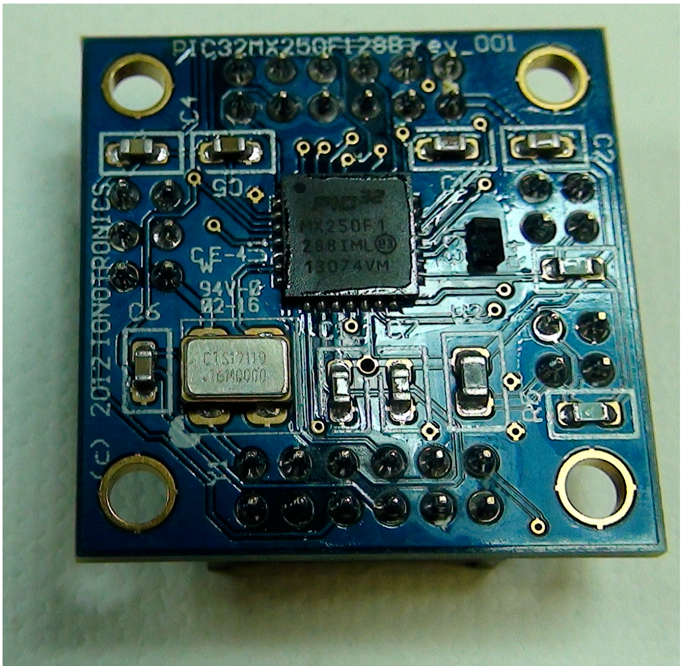
Figure 2 Bottom view of MK-53393 showing PIC32MX250F128 and 16 MHz clock
