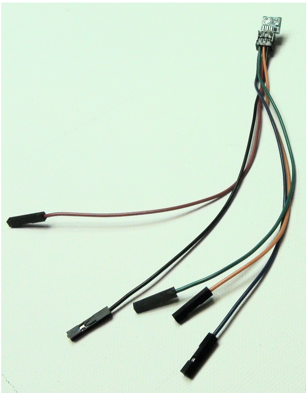
Figure 5 RGB LED with DF-11 4 pin to 25mil Post Cable (MK-76660)
