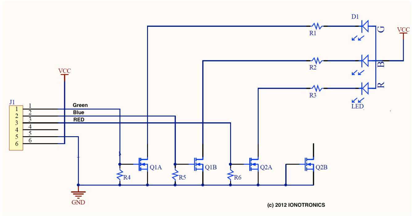
Figure 6 MK-51760 Schematic
