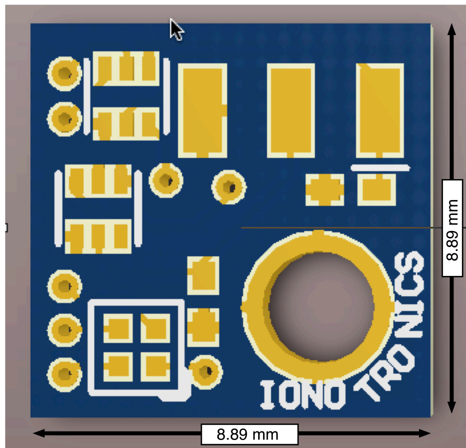
Figure 4 Board Dimensions mm
