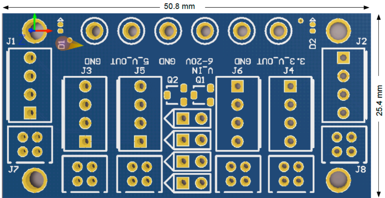
Figure 4 MK-33910 Board Dimensions
