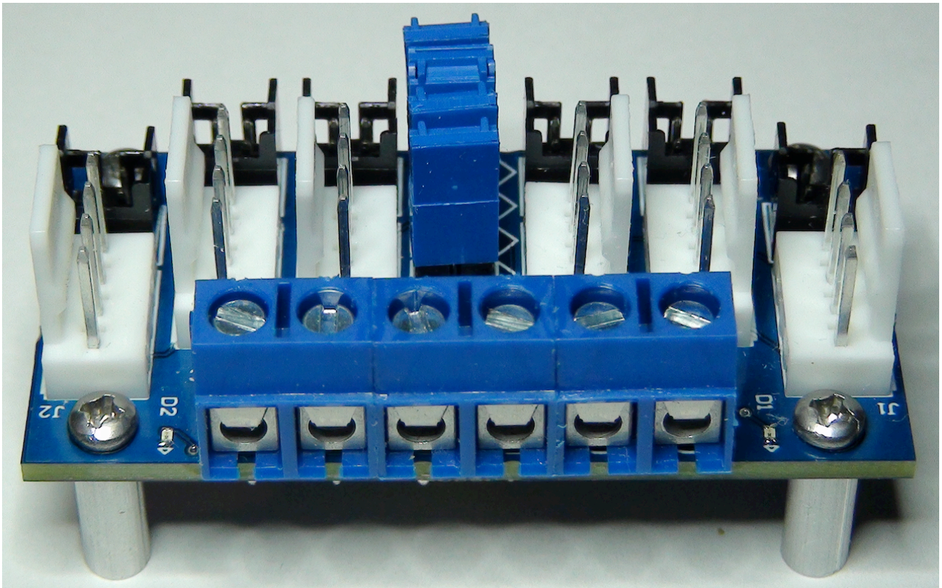
Figure 2 View with Supply Terminals and Standoffs
