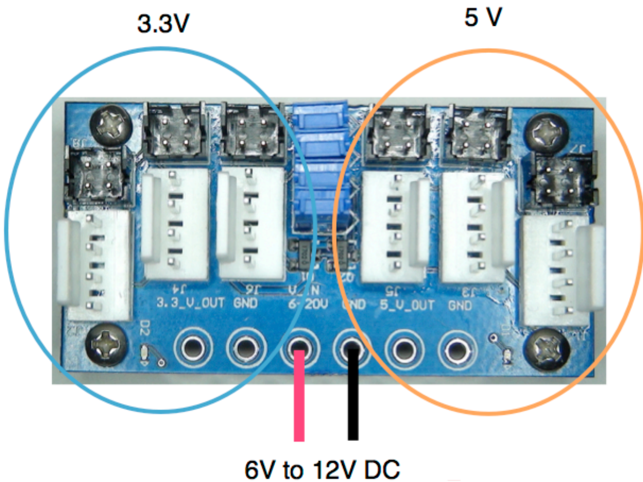
Figure 3 MK-33910 Buss Supply Voltages
