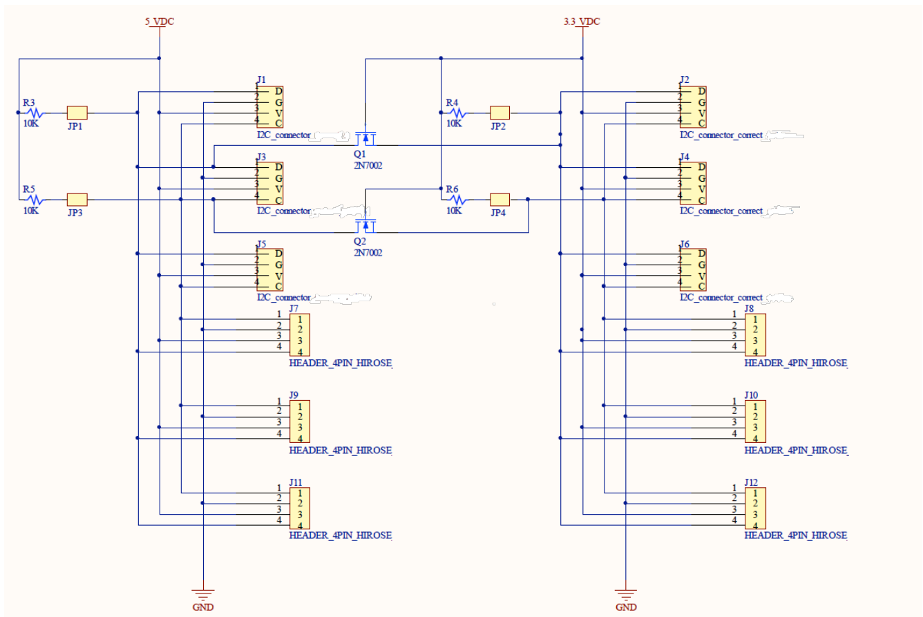
Figure 10 3V and 5V I2C Busses
