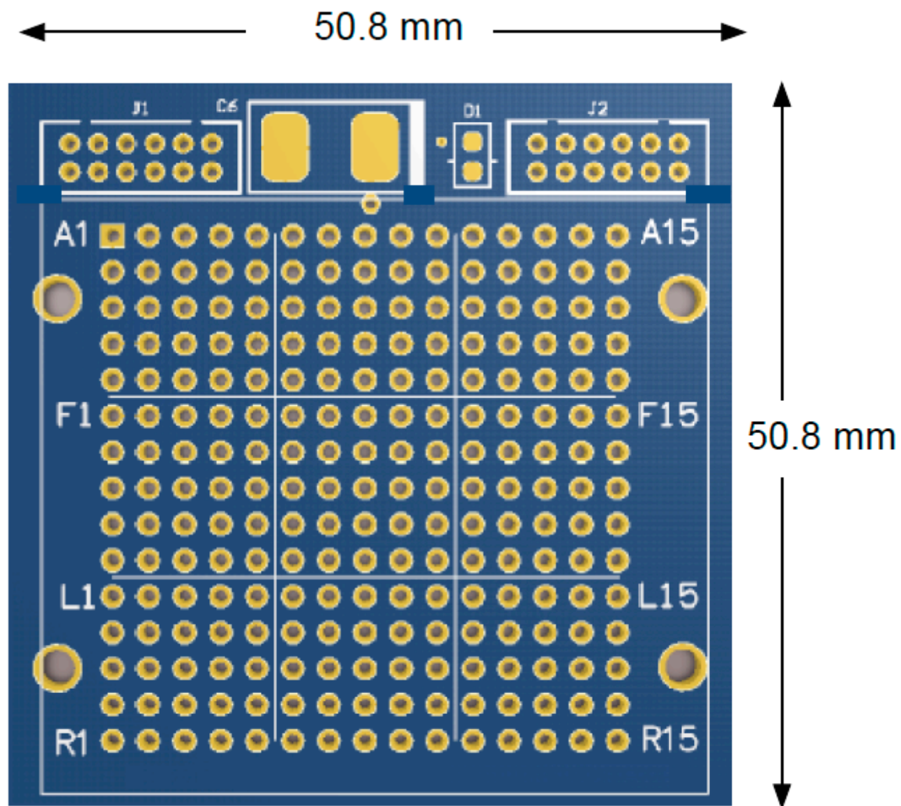
Figure 2 Board Dimensions
