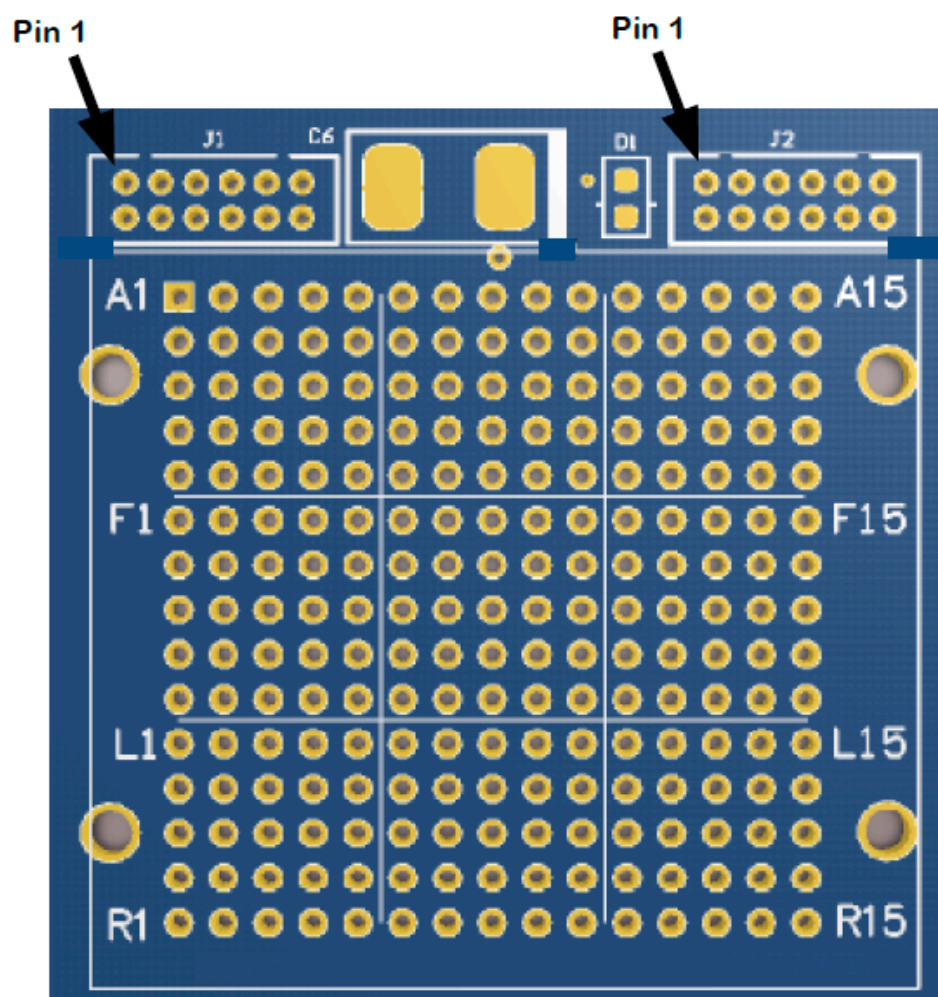
Figure 3 Pin 1 Designation
