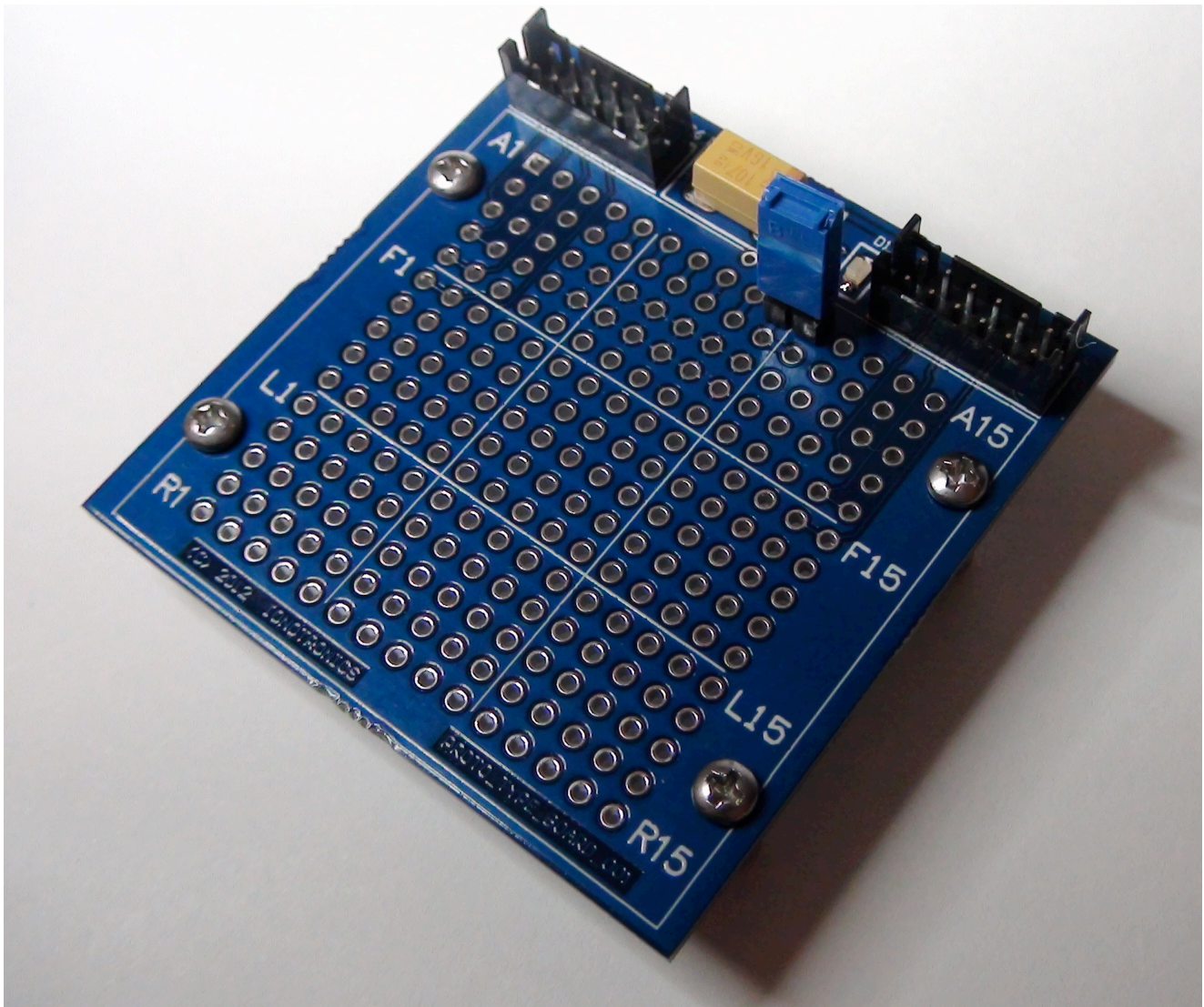
Figure 1 MK-21479 Prototype Board
