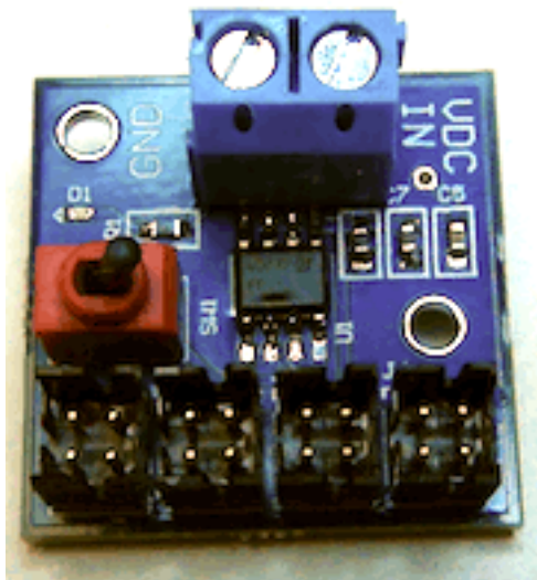
Figure 1 LDO 6V to 5V with 4x I2C Bus Support as Well as 4x 5V Power Source
