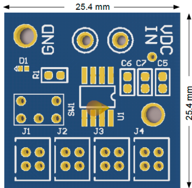
Figure 2 MK-14308 Board Dimensions
